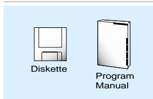
BGVu program
